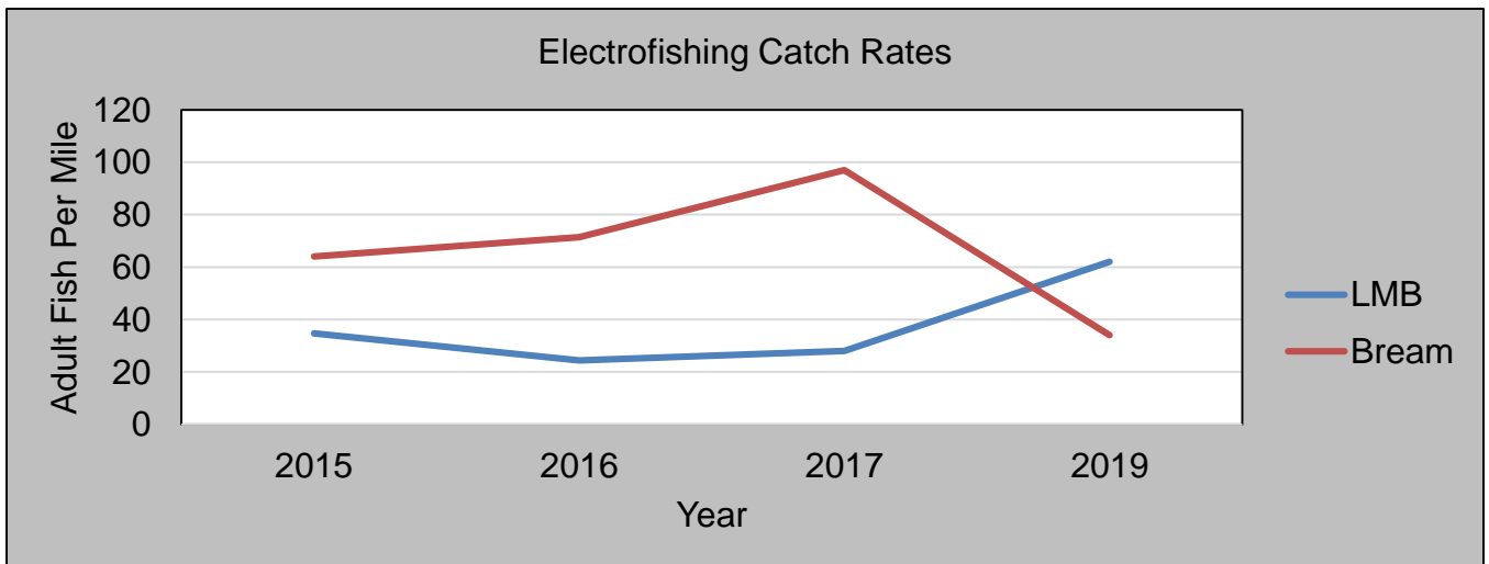
Above: Trends in catch rates during fall electrofishing at Lake Tangipahoa.
