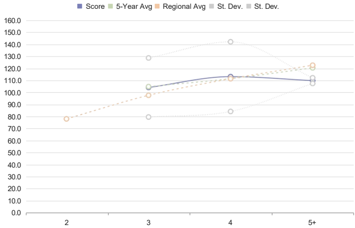
Crieteria B&C Score by Age
