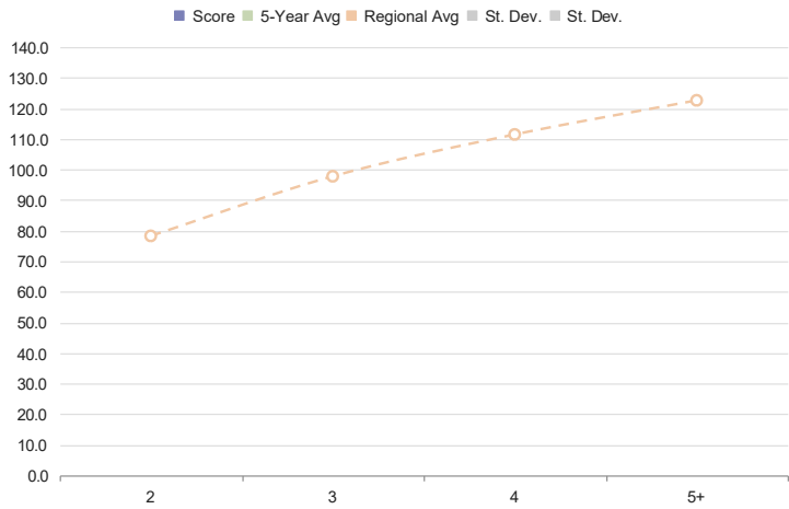
Management Buck B&C Score by Age
