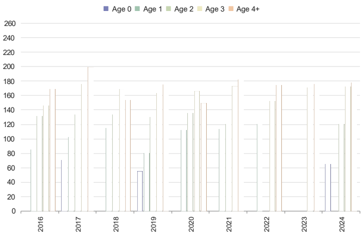
Buck Live Weights
